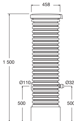
Pumpbrunn
